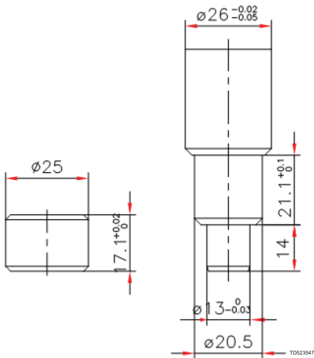
TE81B034: Fixture set f. Collar bush
