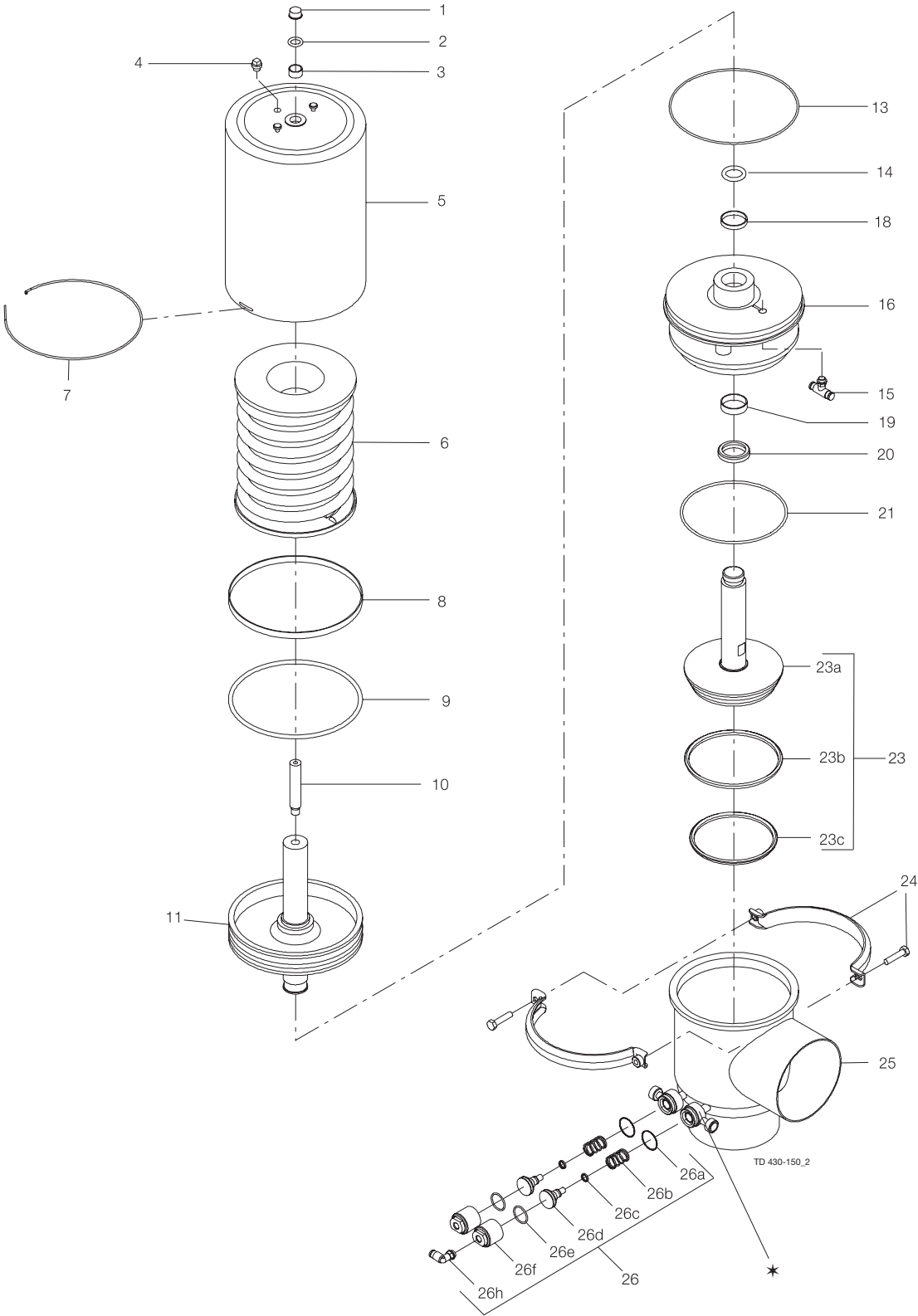
CIP/detecting valve. Diam. ø32.
